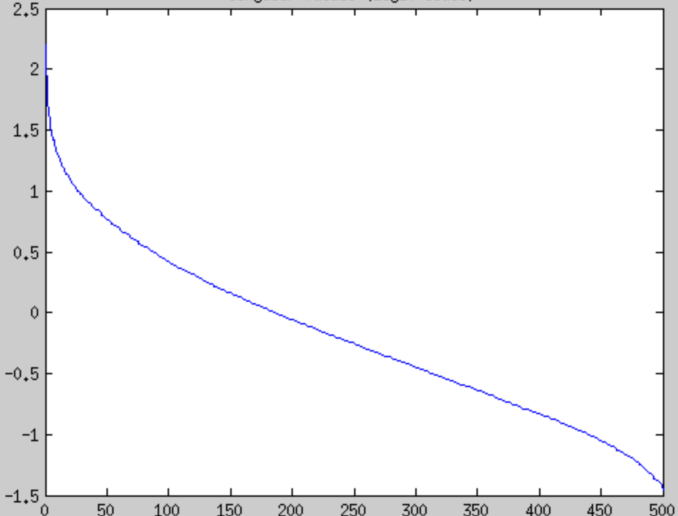
Singular values (Log10 scale)
